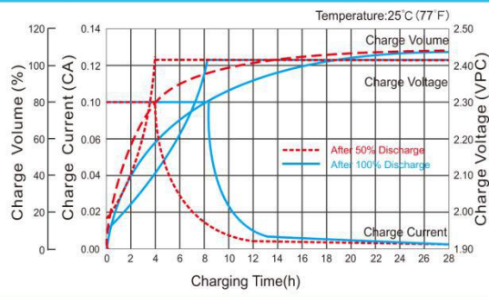
Charge Characteristic Curve for Cycle Use (IU)
