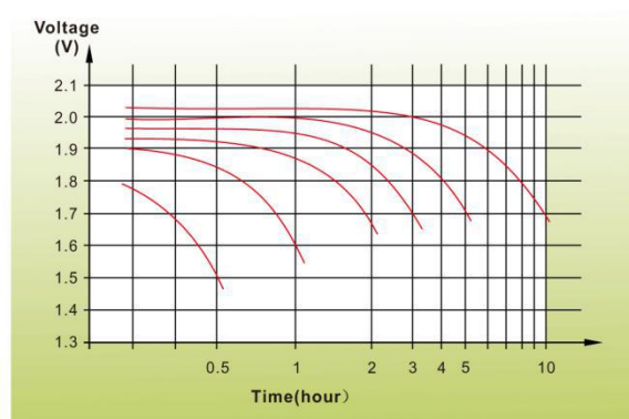
Discharge Characteristics
